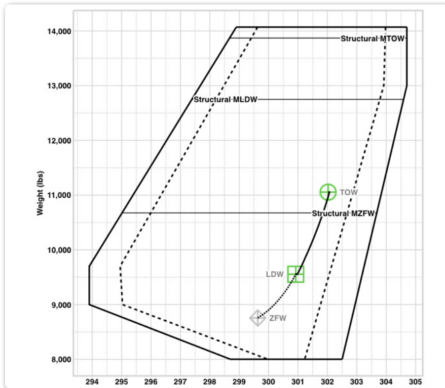
Weight & Balance Curtailed Envelope
