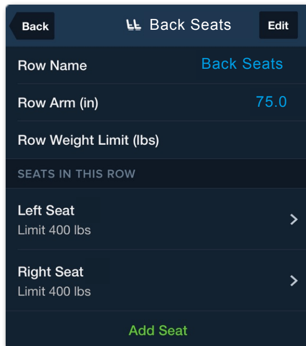
Adding a Row of Seats
